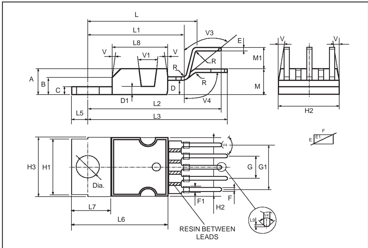
Pentawatt V
