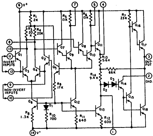
Fig. 1 - Schematic diagram
