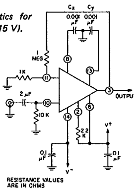
Fig. 8a - Typical 60-dB amplifier.
