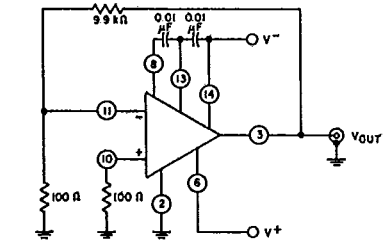
Fig. 2a - Input offset voltage, input offset sensitivity, and device dissipation test circuit.
