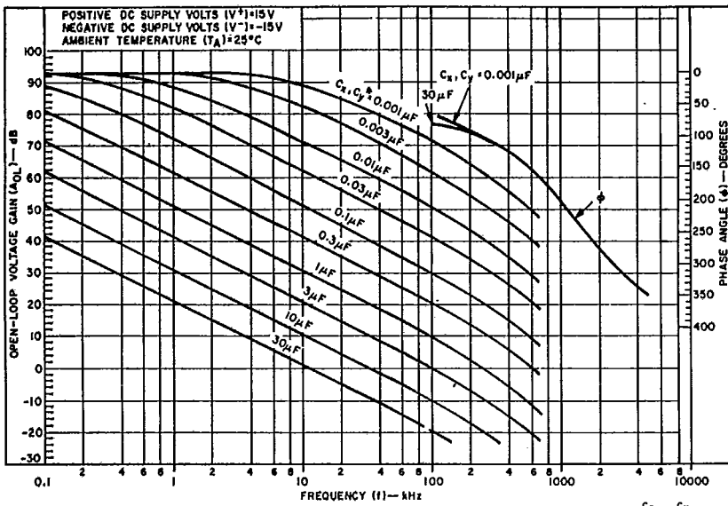
Fig. 8b - Typical phase compensation characteristics for ECG913 ( V^+ = 15\text{ V} , V^- = -15\text{ V} ).
