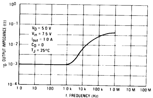
FIGURE 4 — OUTPUT IMPEDANCE
