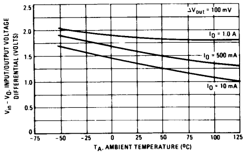
FIGURE 9 — DROPOUT VOLTAGE
