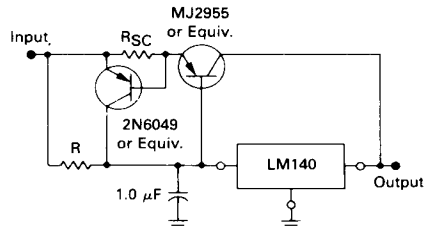
FIGURE 18 — SHORT-CIRCUIT PROTECTION
