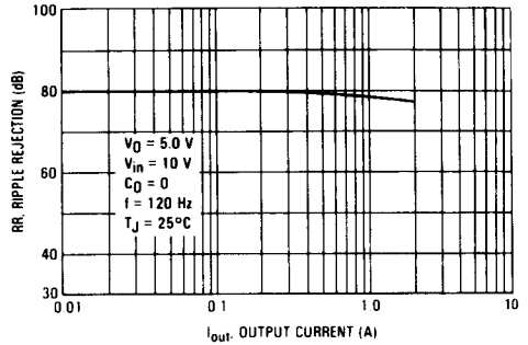
FIGURE 6 — RIPPLE REJECTION versus OUTPUT CURRENT
