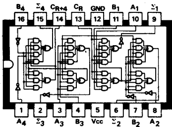
B62 SN7483N 4-bit binary full adder
