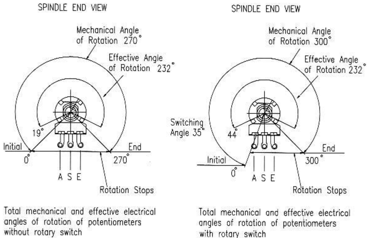
P16 angle of rotation - without and with a rotary switch
