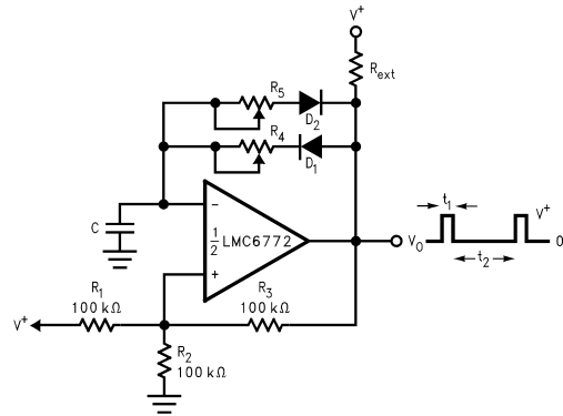
FIGURE 8. Square Wave Generator
