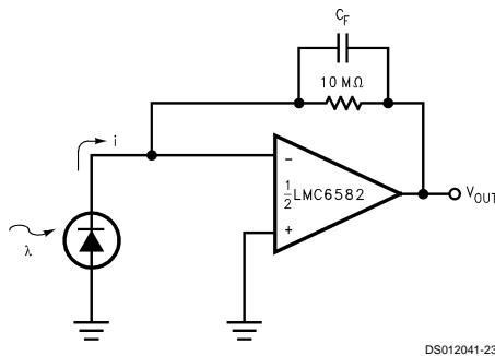
FIGURE 17. Photodiode Amplifier
