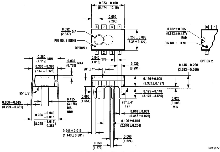
8-Pin Molded Dual-In-Line Package Order Number LMC6081AIN, LMC6081AMN or LMC6081IN NS Package Number N08E
