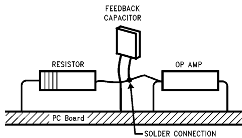
FIGURE 5. Air Wiring
