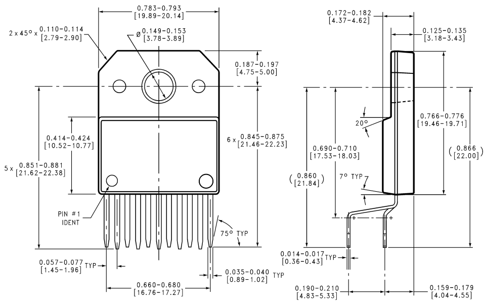
Order Number LM3886TF NS Package Number TF11B
