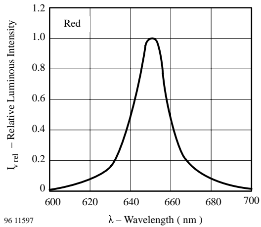
Figure 9 Rel. Luminous Intensity vs. Wavelength
