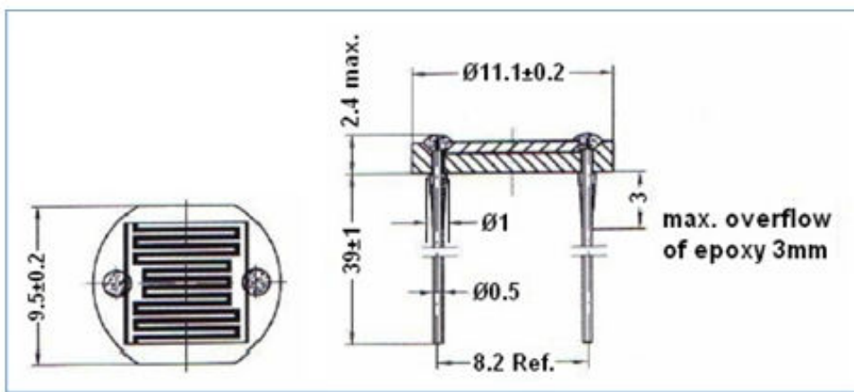
Figure 4 B90... All dimensions in mm
