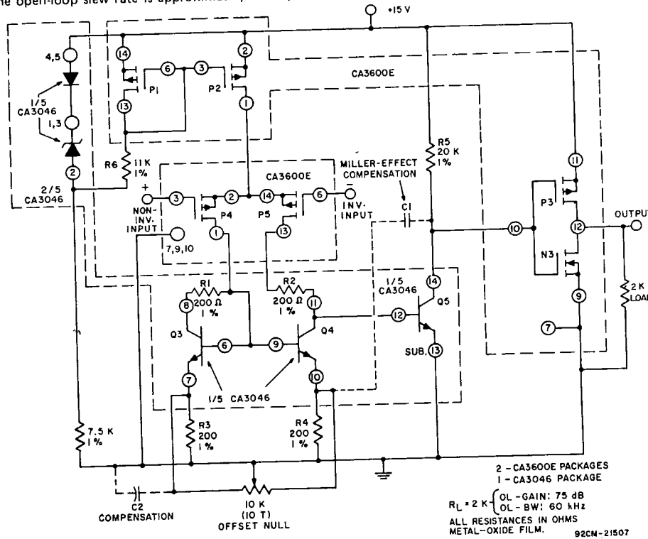
92CN-21507 Fig. 24— Operational amplifier using CMOS transistor-pairs.
