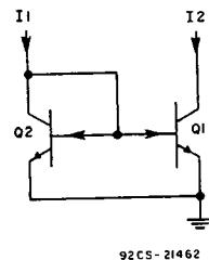
Fig. 28— Current mirror using n-p-n bipolar transistors.
