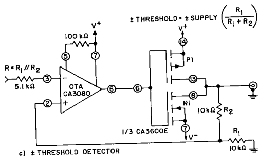
c) ± THRESHOLD DETECTOR
