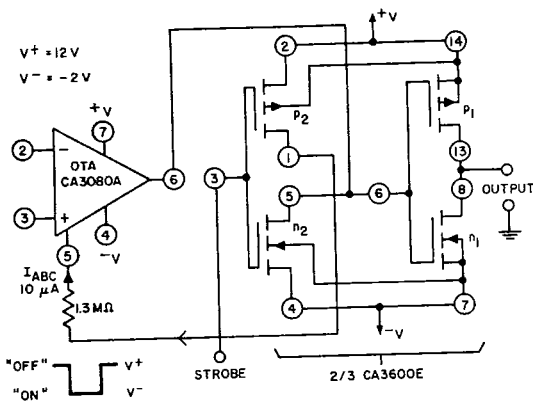
92CS-21535 Fig. 23— Programmable micropower comparator.
