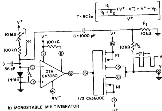
b) MONOSTABLE MULTIVIBRATOR
