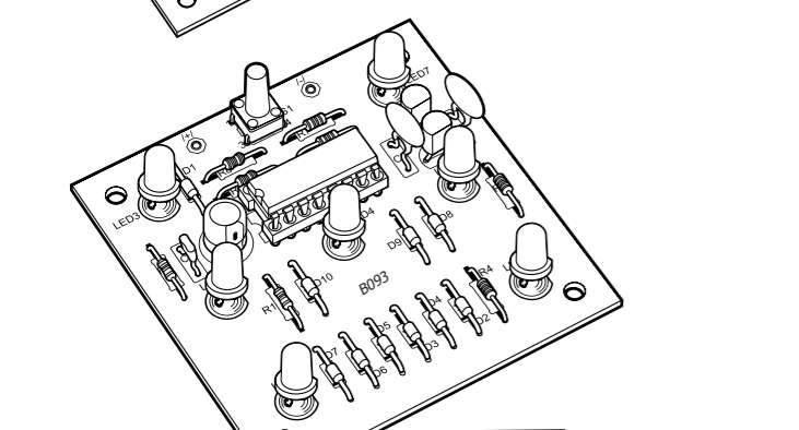
B093 | Electronic Dice | 04-0240P
