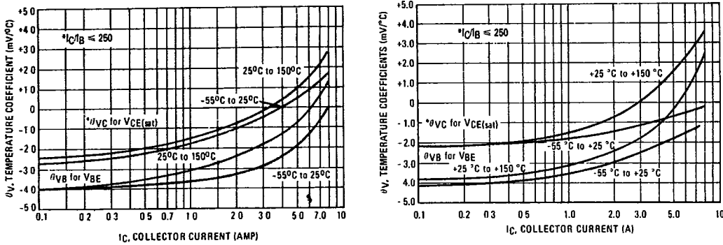
FIGURE 12 - TEMPERATURE COEFFICIENTS
