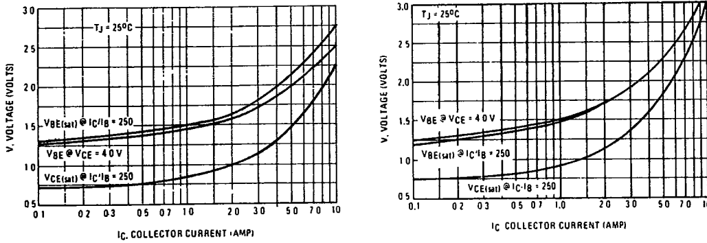
FIGURE 11 - "ON" VOLTAGES
