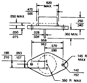
TO-66
