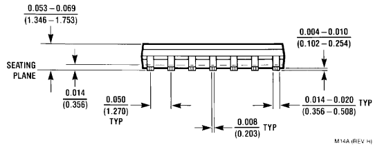
14-Lead Small Outline Integrated Circuit (S) Order Number 74LVQ125SC or 74LVQ125SCX NS Package Number M14A
