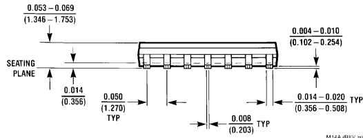
14-Lead (0.150" Wide) Molded Small Outline Package, JEDEC Order Number 74LCX125M or 74LCX125MX NS Package Number M14A
