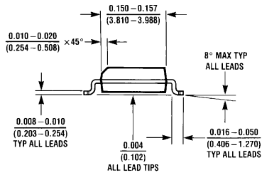
14-Lead (0.150" Wide) Molded Small Outline Package, JEDEC Order Number 74LCX125M or 74LCX125MX NS Package Number M14A
