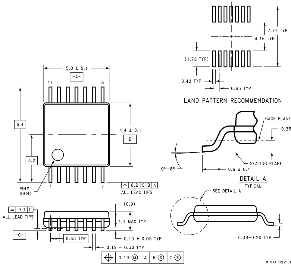
14-Lead Thin Shrink Small Outline Package (MTC) Order Number 74LCX125MTC or 74LCX125MTCX NS Package Number MTC14
