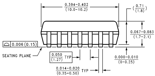
14-Lead (0.300" Wide) Molded Small Outline Package, EIAJ Order Number 74LCX125SJ or 74LCX125SJX NS Package Number M14D
