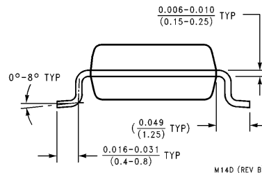
14-Lead (0.300" Wide) Molded Small Outline Package, EIAJ Order Number 74LCX125SJ or 74LCX125SJX NS Package Number M14D
