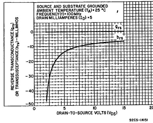
Fig. 10 - Reverse Transadmittance ( y_{rs} ) vs Drain-to-Source Voltage ( V_{DS} )
