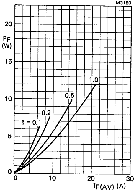
Fig.2 Forward current power rating; per diode.
