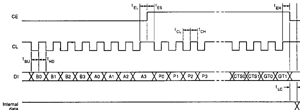
Figure 5. Input timing
