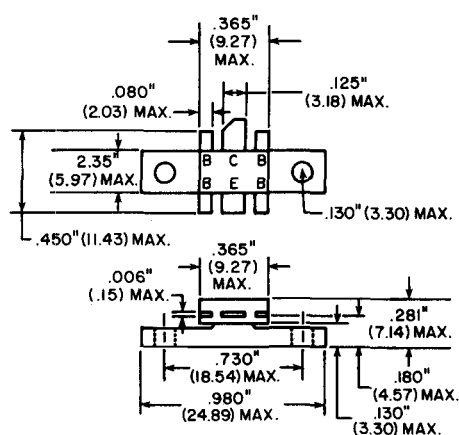
Fig. T62 RF-23F6 ECG 485
