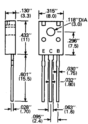
Fig. T69 TO-126M ECG 2501 2502
