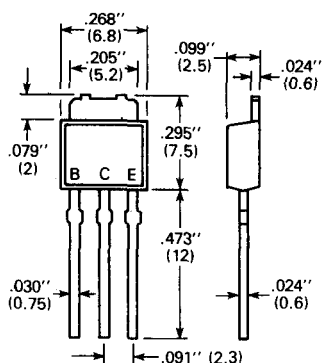
Fig. T70 TO-126N ECG 2351 2352
