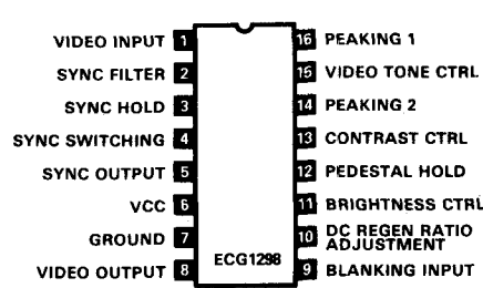
ECG1298 16-Pin DIP See Fig. L111 TV Signal Processor w/Brightness, Contrast Control, Sync Sep
