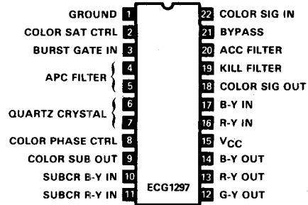
ECG1297 22-Pin DIP See Fig. L121 TV Color Signal Processor/Demodulator
