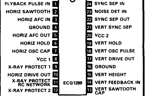
ECG1299 24-Pin DIP See Fig. L122 TV Signal Processor w/V-H Osc, Sync Sep, X-Ray Protect, V CC = 12 V Typ
